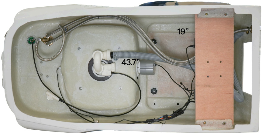
DRAIN PUMP SYSTEM OPTIONAL
